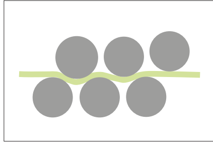
The COMPACT series has 6 manual straightening rollers to remove coil set and give customers flat material every time. The rollers are made of polished steel with a 2.75" (70 mm) diameter.
